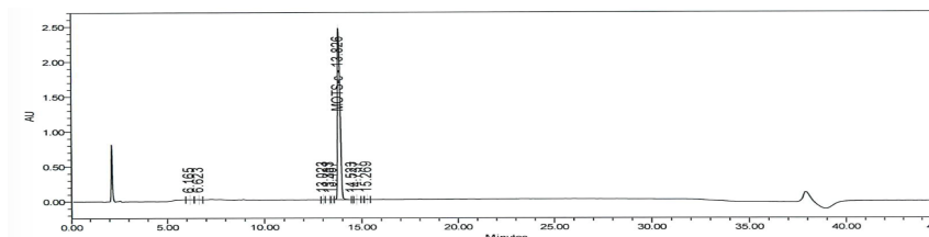
HPLC-UV Chromatogram
