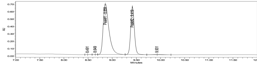
HPLC-UV Chromatogram
